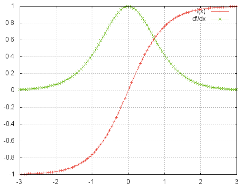
Diagram 4: Graphs of tanh and its derivative 1
