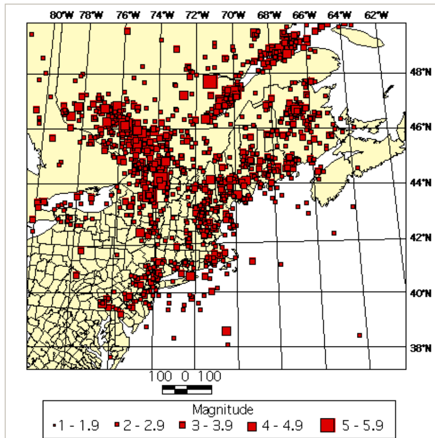
Figure 4: Seismicity for period October, 1975 - June, 2002.
