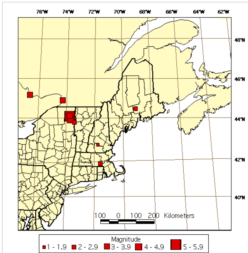
Figure 3: Earthquake epicenters located by the NESN during period April - June, 2002.
